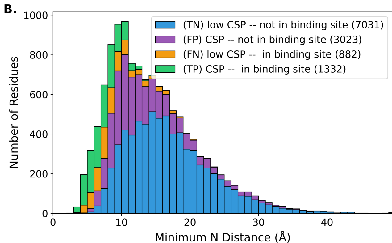
SI Fig. S12. Confusion histograms by closest interchain N–N distance ( n = 135 buffer-similar systems from CSP_UBQ_ph0.5_temp5C.csv with pipeline outputs).
