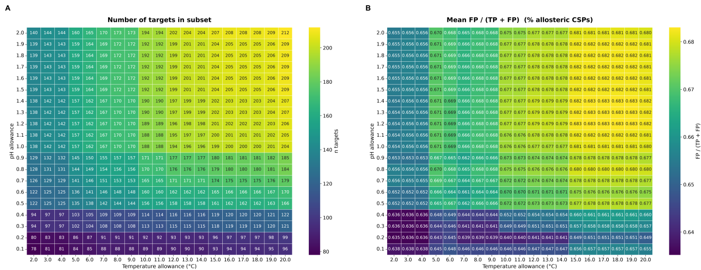
SI Fig. S20. Buffer pH/temperature threshold sweep. (A) Number of apo/holo pairs retained as |\Delta\text{pH}| and |\Delta T| thresholds are tightened. (B) Mean FP/(TP+FP) (percent allosteric CSPs) in the same subsets.
