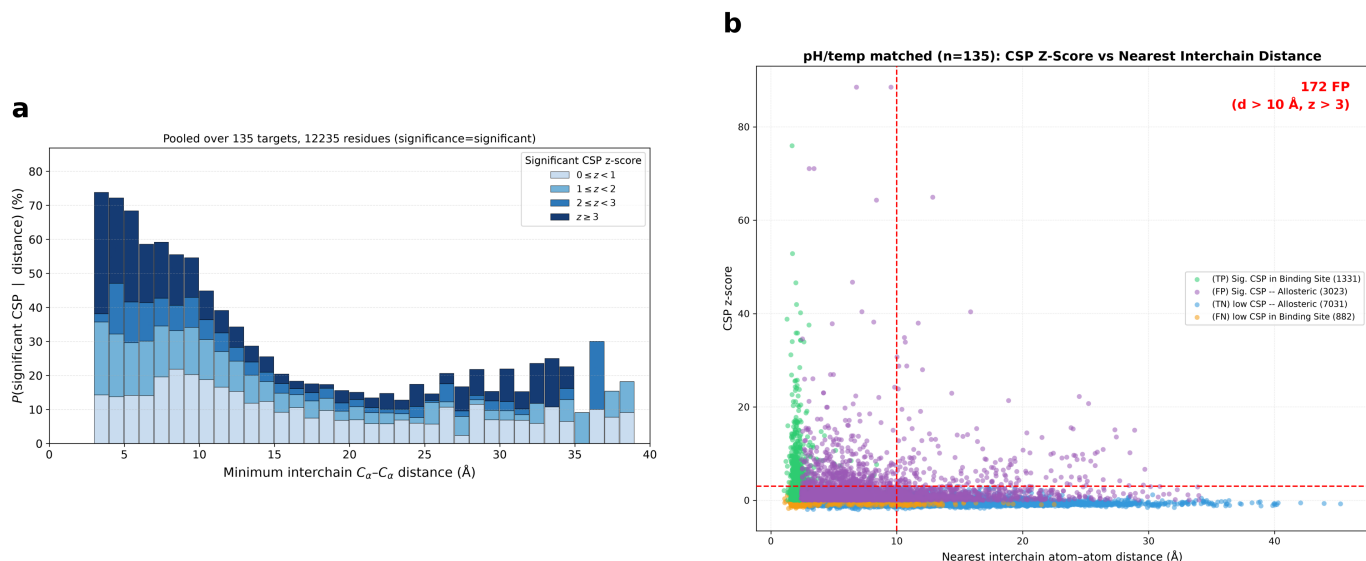
SI Fig. S17. Chemical-shift perturbations as a function of interchain distance. (a) Residue-pooled P(\text{significant CSP} \mid \text{minimum interchain } C_\alpha\text{-}C_\alpha \text{ distance}) for buffer-similar systems ( n = 135 from CSP_UBQ_ph0.5_temp5C.csv with pipeline outputs) under the primary cutoff \max(\text{cleaned mean}, 0.05 \text{ ppm}) . Bar height is the fraction of residues with a recorded HN CSP that are called significant in each 1 \text{ \AA} distance bin; stacks partition those significant CSPs by cleaned-mean z -score ( 0 \leq z < 1 , 1 \leq z < 2 , 2 \leq z < 3 , z \geq 3 ). Close to the interface the significant fraction is high and enriched in large z , then declines toward a lower baseline at longer range. (b) Per-residue CSP z -score versus nearest interchain any-atom distance for the same n = 135 set (same primary significance definition), colored by confusion-matrix class (TP/FP/TN/FN) relative to the structural binding-site mask. Dashed lines mark z = 3 and d = 10 \text{ \AA} ; the annotation counts false positives with d > 10 \text{ \AA} and z > 3 .
