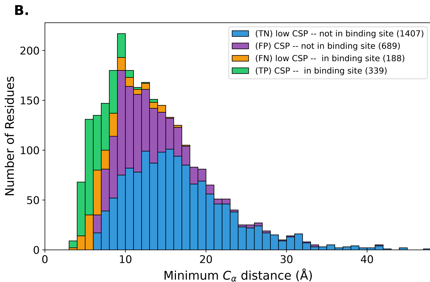
SI Fig. S16. Figure 3 histograms for the same-author/same-study subset. Targets are the curated pairs in CSP_UBQ_ph0.5_temp5C_same_author_list.csv ( n = 32 with pipeline outputs of 33 curated pairs): buffer-similar apo/holo systems that share a study or last author between apo and holo chemical-shift depositions. Left: significant-CSP TP vs FP by minimum C_{\alpha} distance to the interface; right: full confusion-matrix
