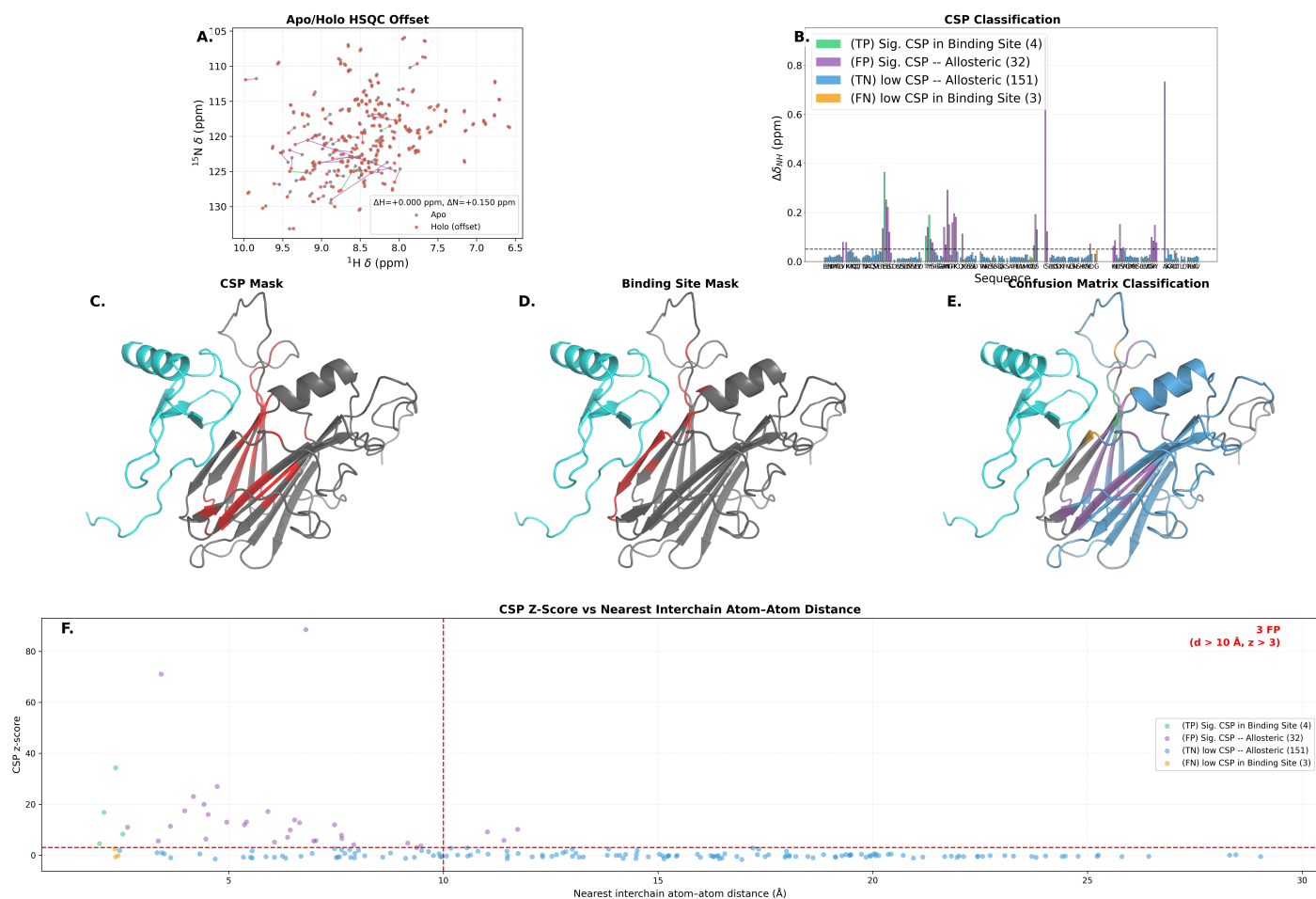
SI Fig. S18. Case study for holo 2FIN / apo BMRB 6809 (holo BMRB 7024). HSQC overlay, CSP classification bars, CSP / binding-site / confusion structure views, and CSP z versus nearest interchain atom–atom distance. (F) Dashed lines mark z = 3 and d = 10 \text{ \AA} ; the annotation counts false positives with d > 10 \text{ \AA} and z > 3 . This plot shows monotonic decay of CSPs with increasing nearest interchain atom–atom distance. Residues in a set of \beta sheets further away from the ligand with significant shifts have lower CSPs than those closer to the binding site.
