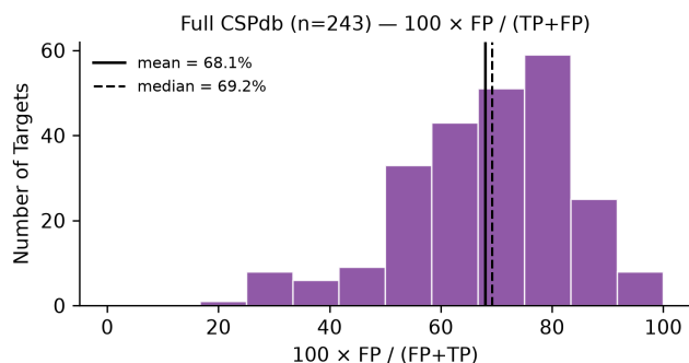
SI Fig. S15. Per-target false-positive rates under the primary CSP cutoff max(cleaned mean, 0.05 ppm). Rows show four cohorts: ideal sequence match ( n = 83 ), non-ideal sequence match ( n = 52 ), pH/temp matched ( n = 135 ), and the full CSPdb ( n = 243 ). For each cohort, panels report 100 \times \text{FP} / (\text{TP} + \text{FP}) among significant CSPs.
