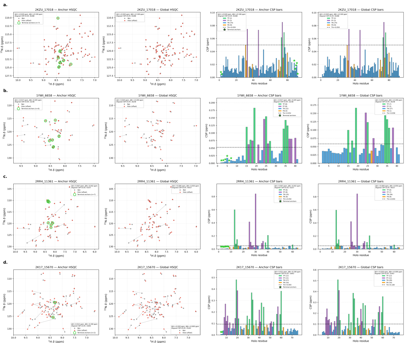
SI Fig. S22. Terminal-anchor vs global offsets: HSQC overlays and CSP classification bars for four targets (2KZU/17018, 1YWI/6658, 2RR4/11361, 2K17/15670). For each target (rows a–d): left pair shows apo (grey) vs offset holo (red) HSQC overlays using terminal-anchor RMSD offsets vs the global CSP-count grid; right pair shows corresponding CSP classification bars (TP/FP/TN/FN) under the primary significance threshold. Green markers denote terminal-anchor residues.
