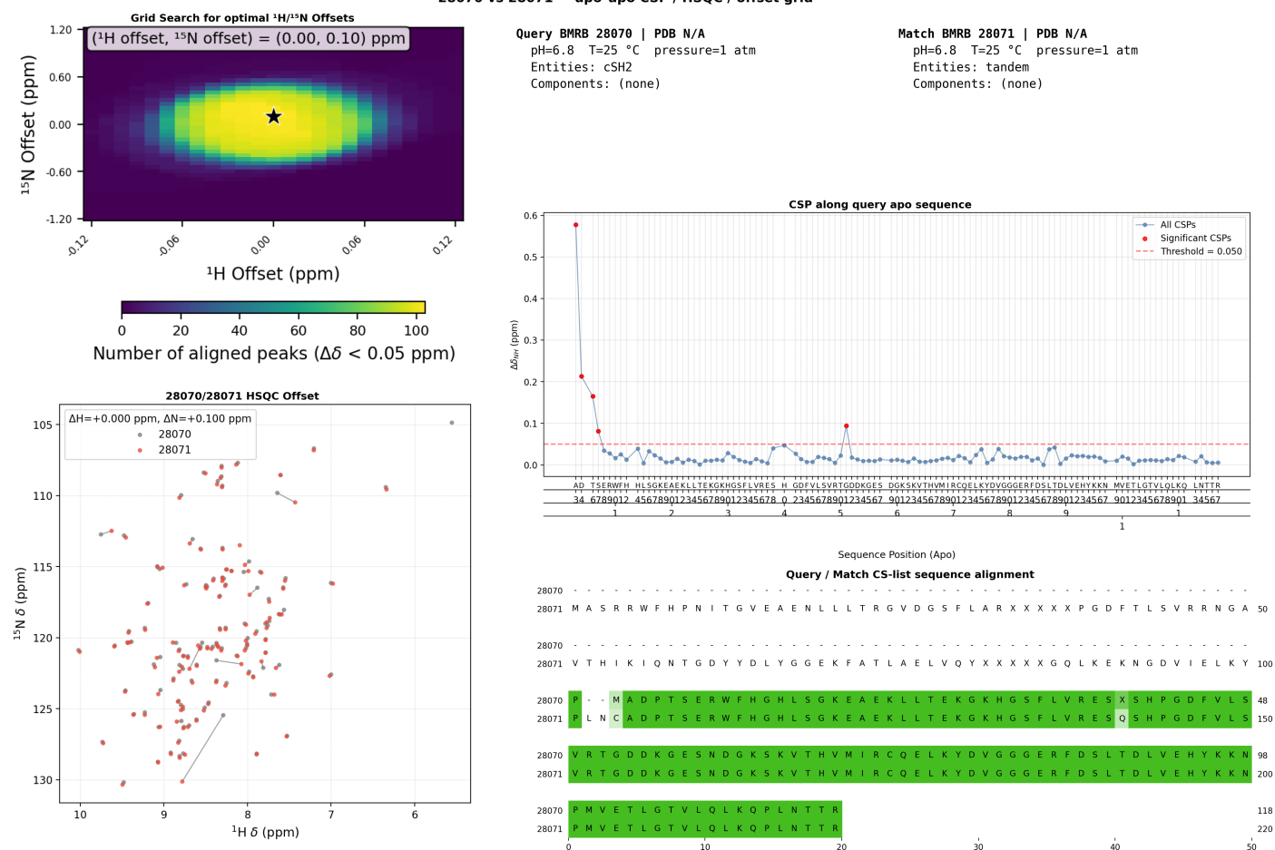
SI Fig. S25B. Apo vs apo control study for BMRB 28070 and 28071. This case involves the SH2 domains of SHP2. BMRB 28071 is the tandem nSH2–cSH2 construct and includes a large N-terminal region (the nSH2 domain and inter-SH2 linker, ~100 residues) that is absent from the isolated cSH2 entry (BMRB 28070). 95.4% of the CSPs for this control are below 0.05 ppm.
