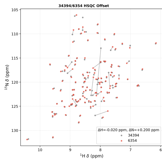
SI Fig. S25D. Apo vs apo control study for BMRB 34394 and 6354. This case involves the NECAP1 Phear domain. BMRB 34394 has a five-residue N-terminal extension (GSPNS) relative to BMRB 6354, plus substitutions T8A and K59I and short internal insertions (Pro28 and Ala31–Ser32) in the 34394 construct. 83.2% of the CSPs for this control are below 0.05 ppm.
